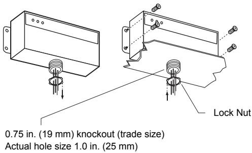
Figure 4: Mounting Unit
