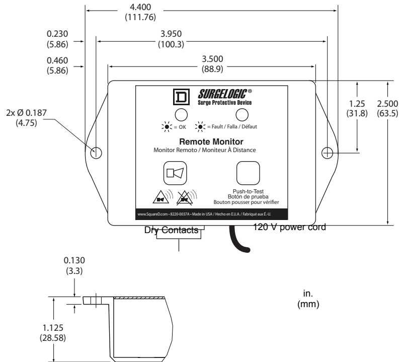
Figure 10: Remote Monitor Option (TVS12RMU)
